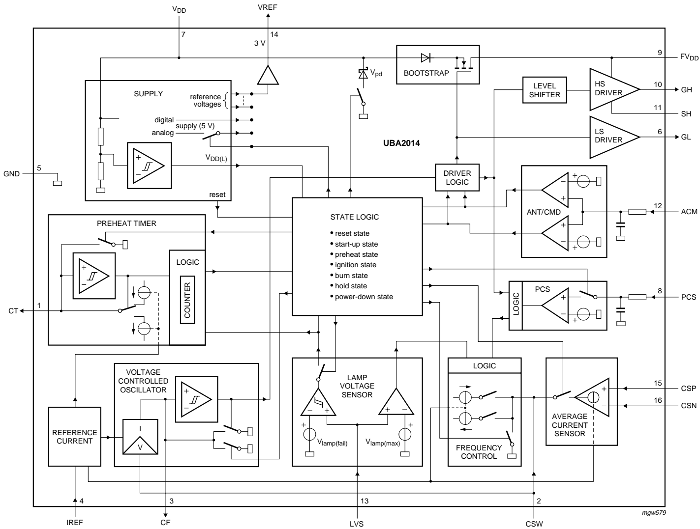
Fig 1. Block diagram
